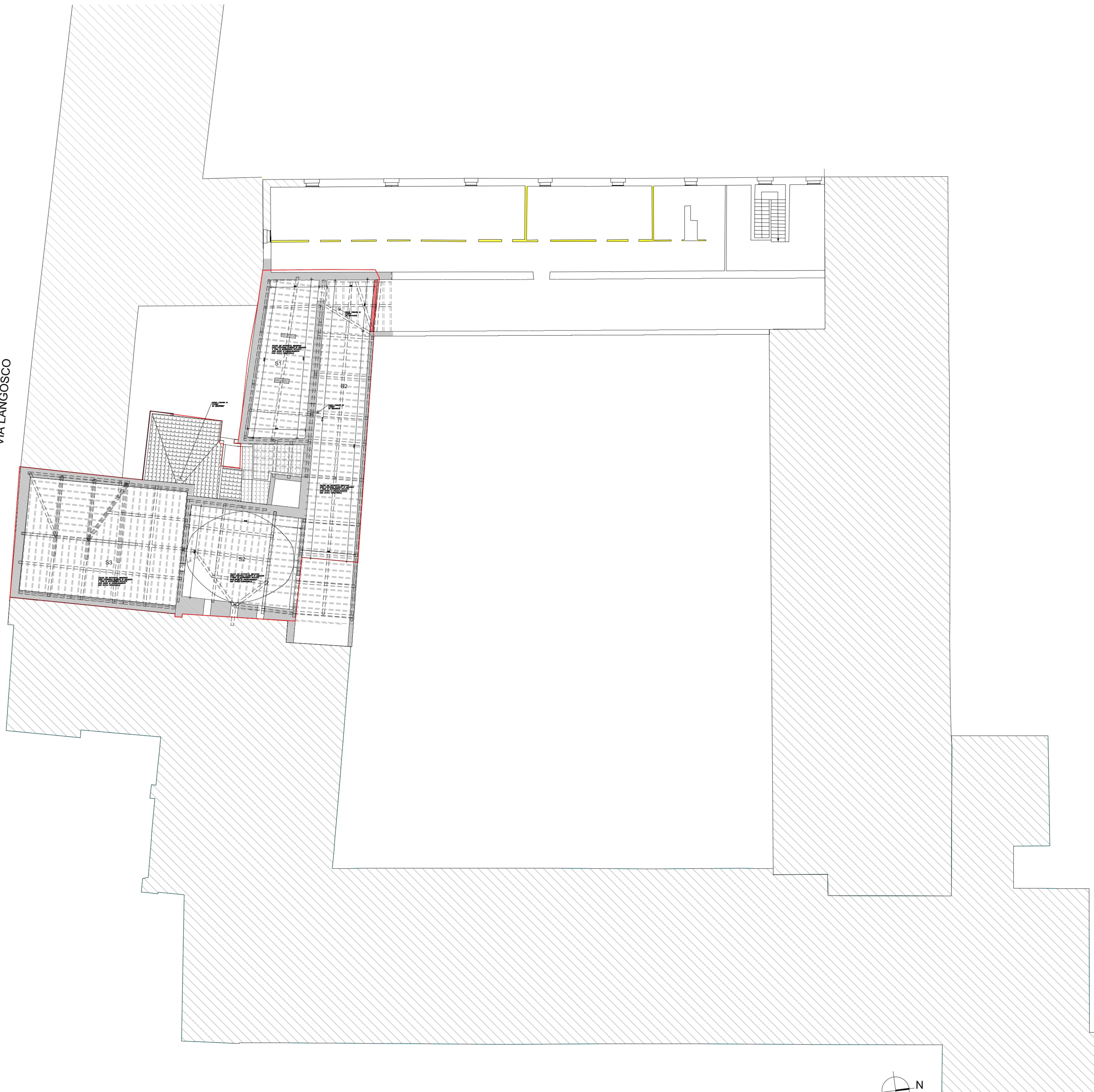
KEY PLAN
