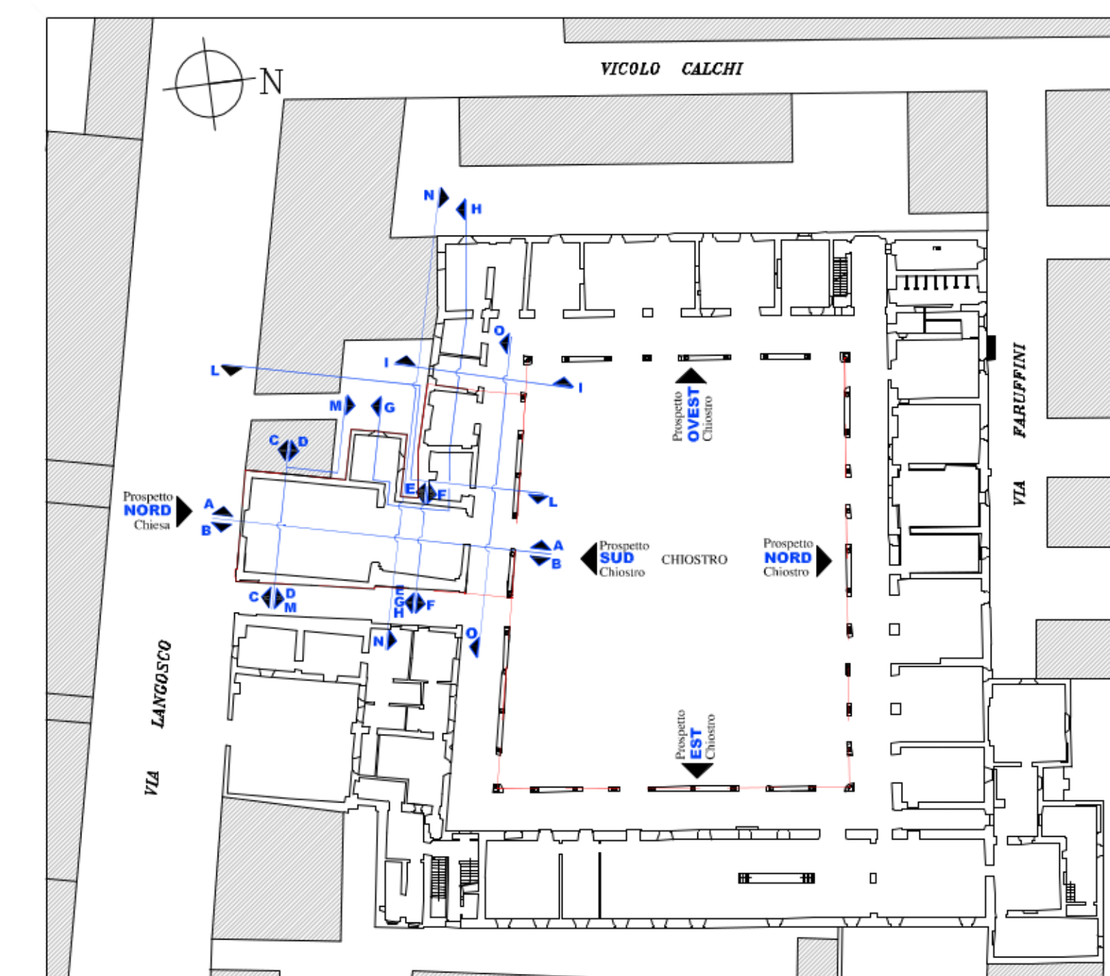
KEY PLAN
